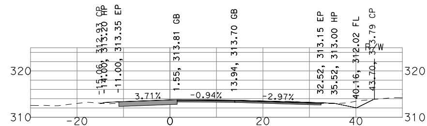
"GSB_R3_NB4" 459+00
