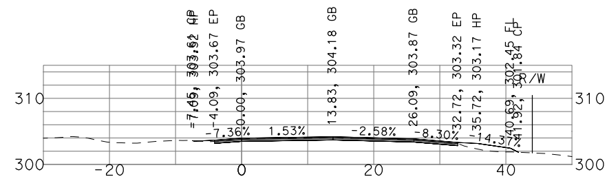
"GSB_R3_NB4" 501+00
