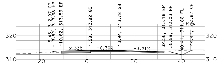
"GSB_R3_NB4" 458+50
