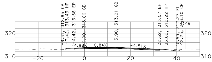
"GSB_R3_NB4" 456+50
