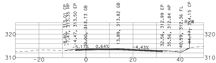
"GSB_R3_NB4" 456+00
