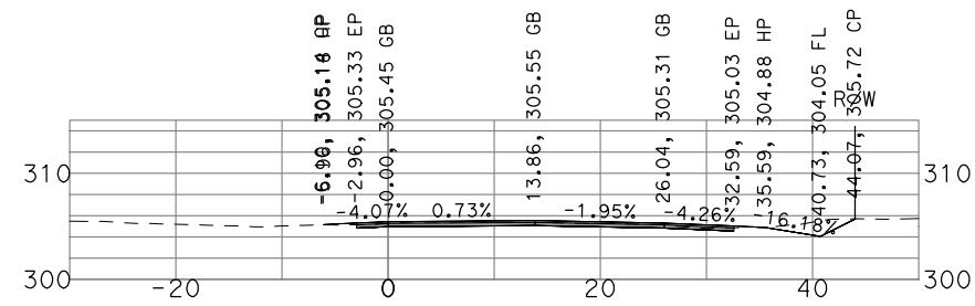
"GSB_R3_NB4" 504+00
