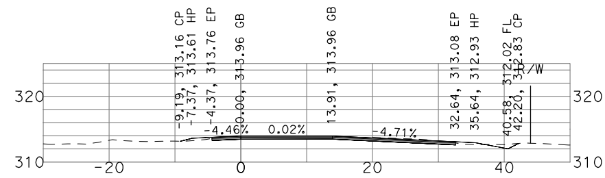
"GSB_R3_NB4" 457+00
