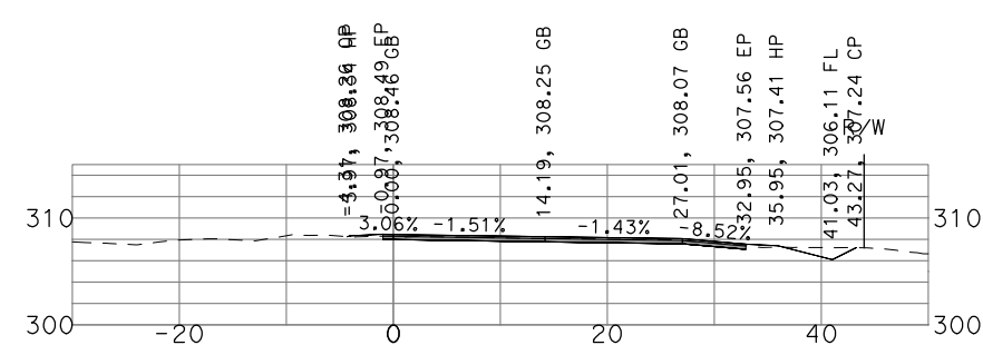
"GSB_R3_NB4" 526+50
