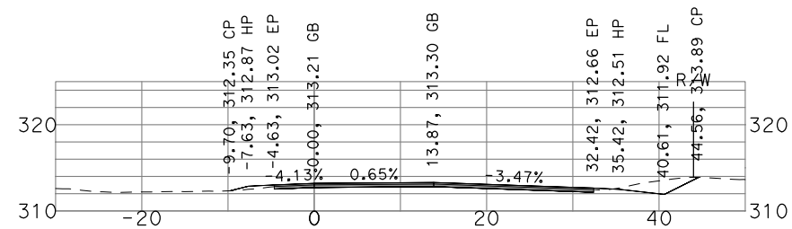
"GSB_R3_NB4" 454+50
