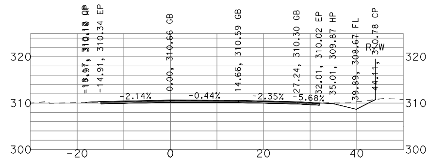
"GSB_R3_NB4" 540+50
