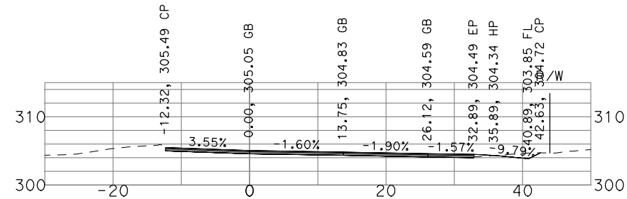
"GSB_R3_NB4" 492+50
