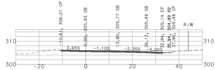
"GSB_R3_NB4" 491+50
