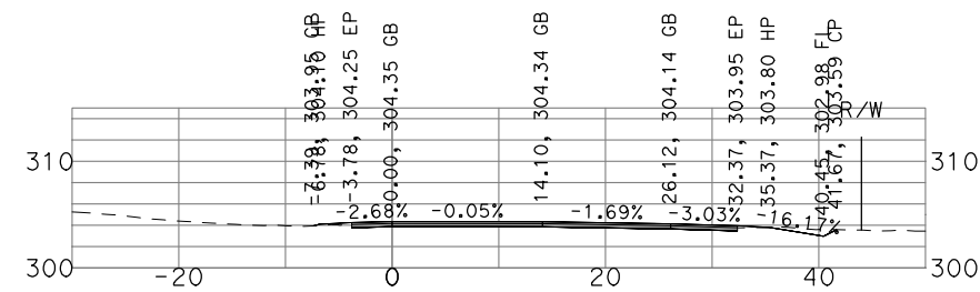
"GSB_R3_NB4" 482+00
