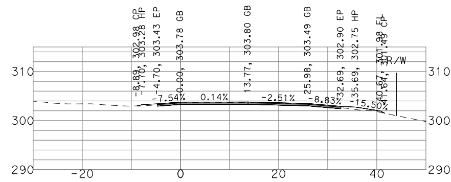
"GSB_R3_NB4" 499+50
