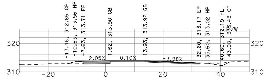
"GSB_R3_NB4" 458+00
