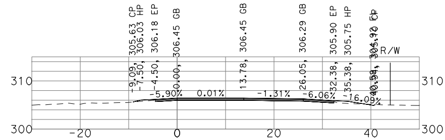
"GSB_R3_NB4" 489+50
