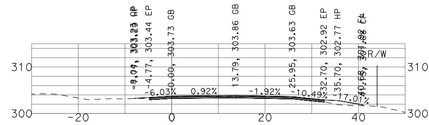
"GSB_R3_NB4" 500+00
