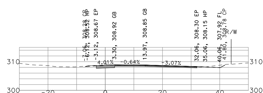
"GSB_R3_NB4" 466+50
