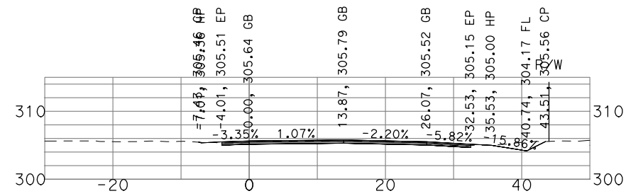
"GSB_R3_NB4" 504+50
