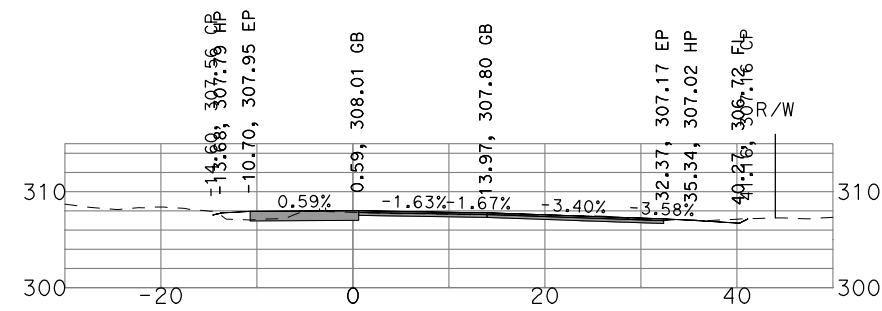
"GSB_R3_NB4" 467+50
