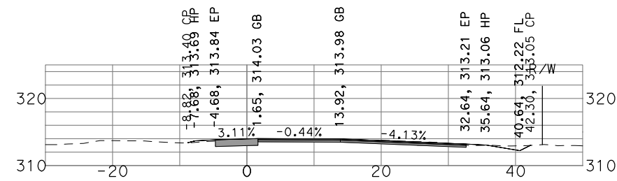
"GSB_R3_NB4" 457+50
