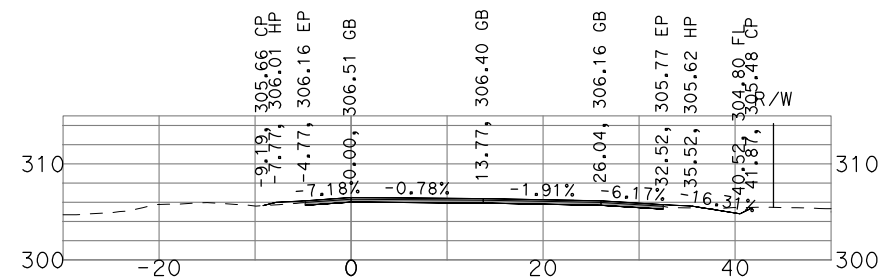
"GSB_R3_NB4" 489+00
