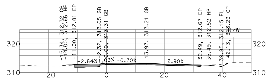
"GSB_R3_NB4" 460+50
