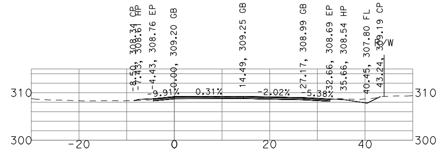
"GSB_R3_NB4" 537+50
