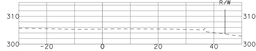
"GSB_R3_NB4" 479+00
