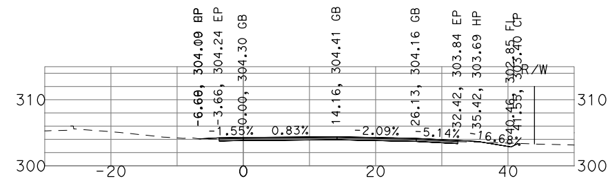
"GSB_R3_NB4" 481+50
