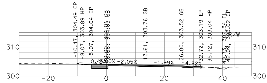
"GSB_R3_NB4" 496+00
