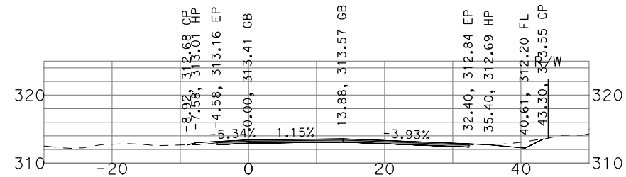
"GSB_R3_NB4" 455+00
