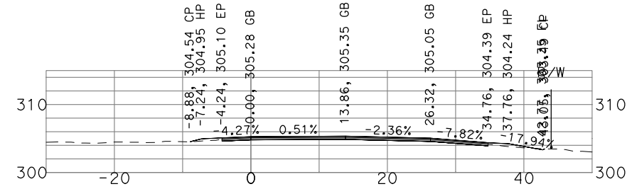
"GSB_R3_NB4" 485+50
