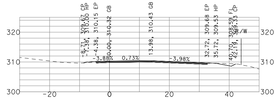
"GSB_R3_NB4" 448+00
