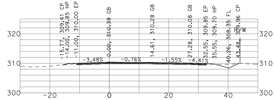
"GSB_R3_NB4" 539+50
