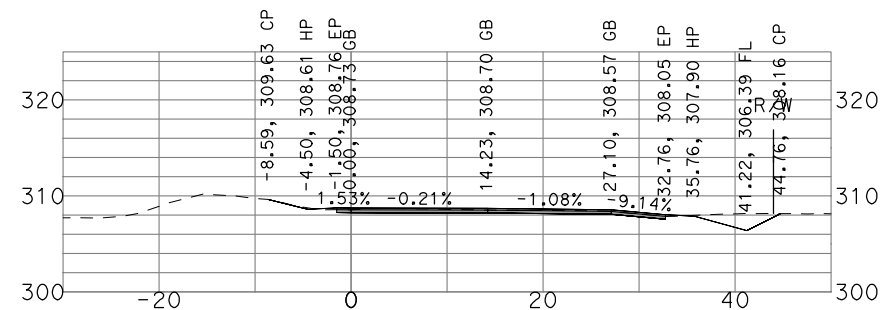
"GSB_R3_NB4" 525+00
