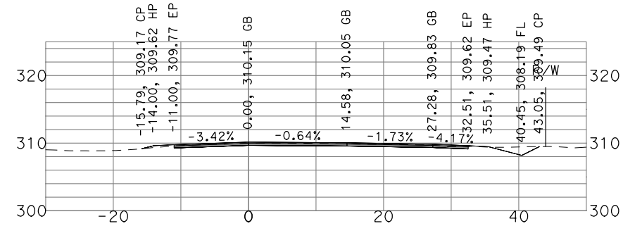
"GSB_R3_NB4" 539+00
