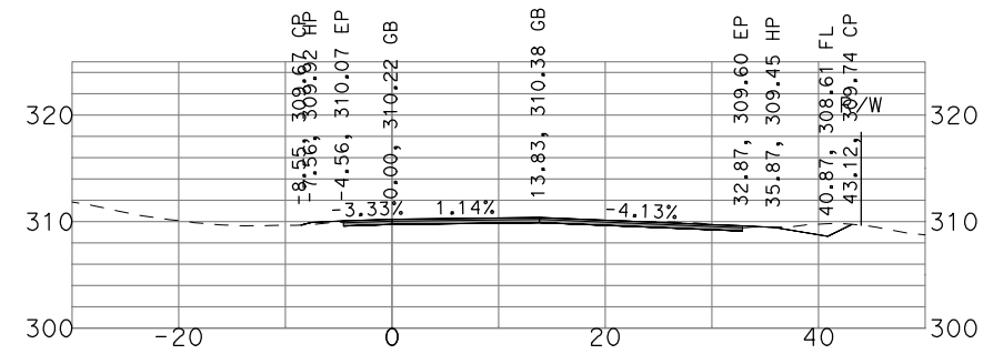
"GSB_R3_NB4" 449+50
