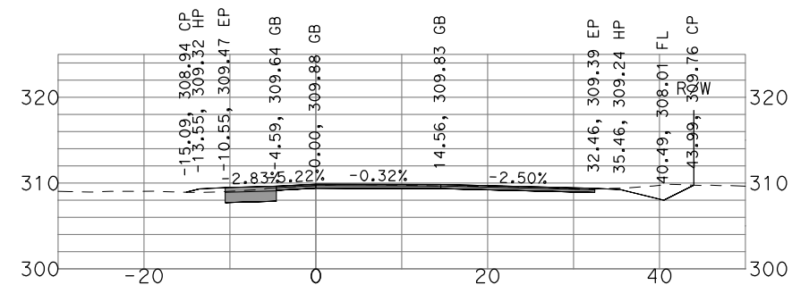
"GSB_R3_NB4" 538+50
