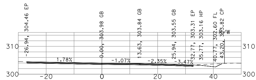
"GSB_R3_NB4" 495+00
