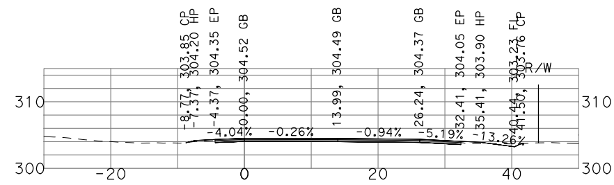
"GSB_R3_NB4" 483+00
