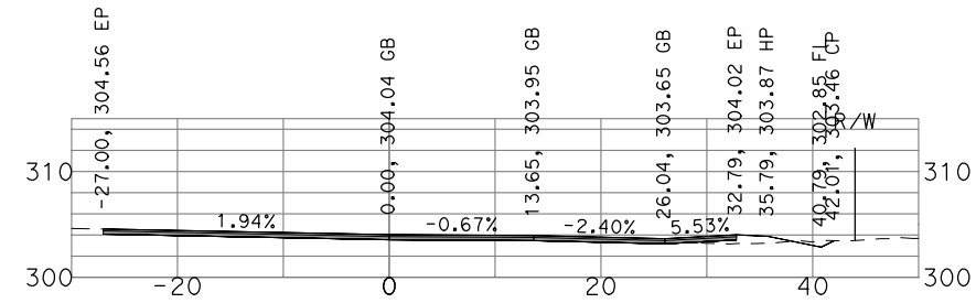
"GSB_R3_NB4" 494+50
