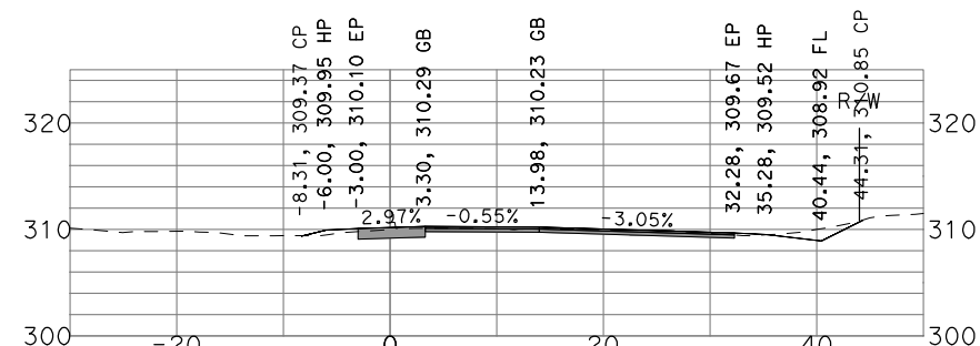
"GSB_R3_NB4" 465+00
