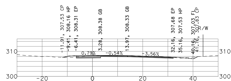
"GSB_R3_NB4" 467+00
