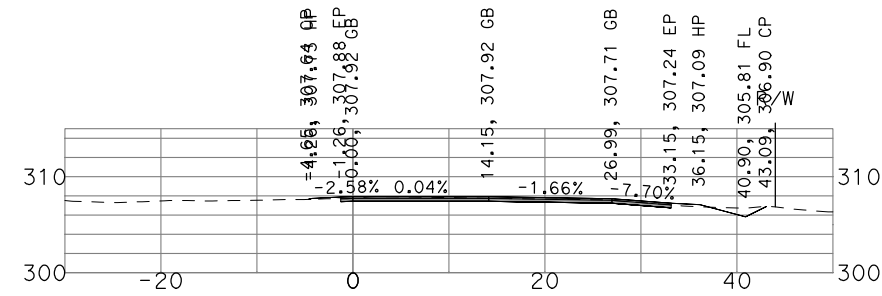
"GSB_R3_NB4" 527+50
