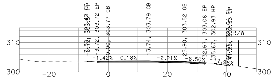
"GSB_R3_NB4" 499+00
