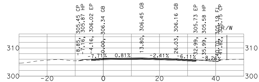
"GSB_R3_NB4" 490+50
