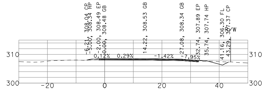
"GSB_R3_NB4" 525+50
