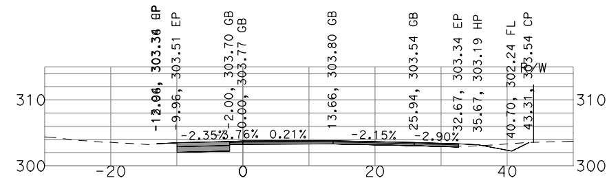
"GSB_R3_NB4" 497+00
