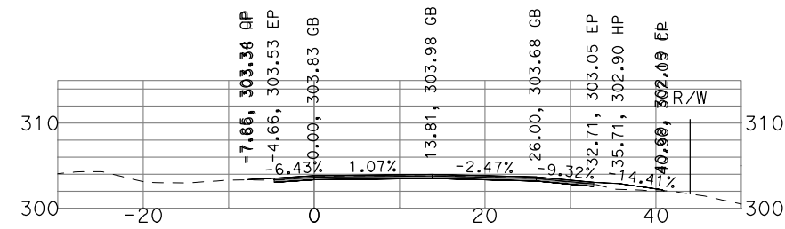
"GSB_R3_NB4" 500+50
