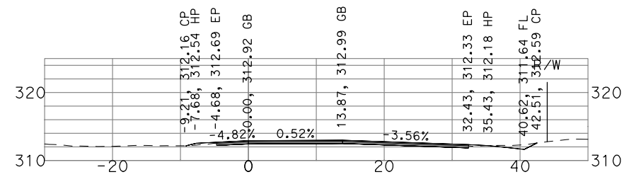
"GSB_R3_NB4" 454+00
