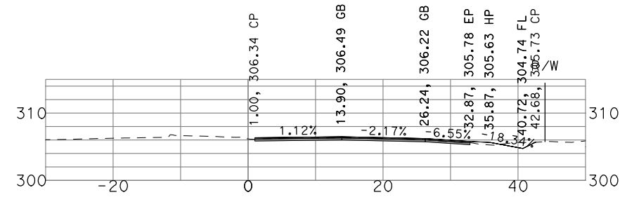
"GSB_R3_NB4" 506+00
