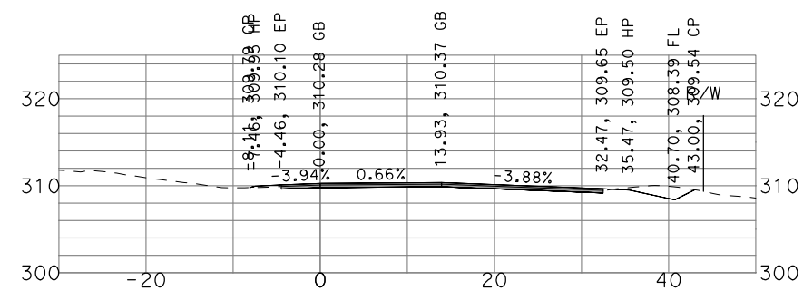
"GSB_R3_NB4" 448+50
