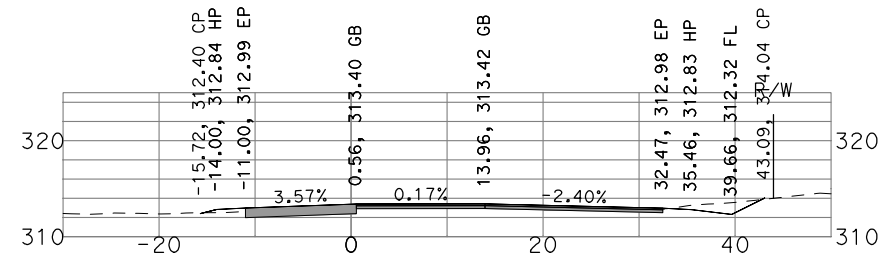
"GSB_R3_NB4" 460+00
