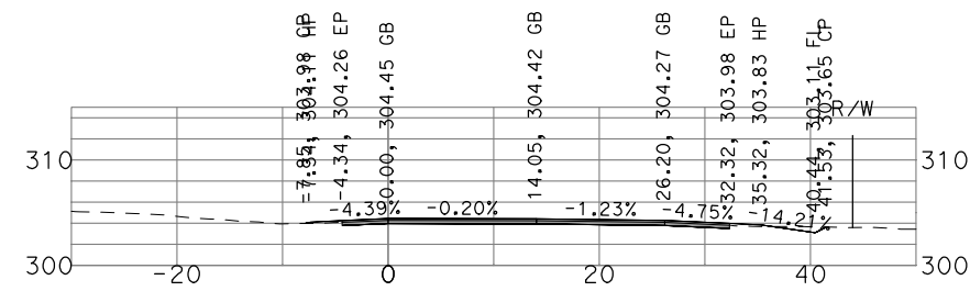
"GSB_R3_NB4" 482+50
