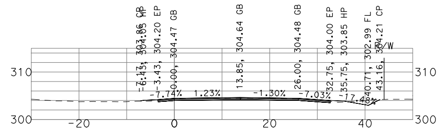
"GSB_R3_NB4" 502+00
