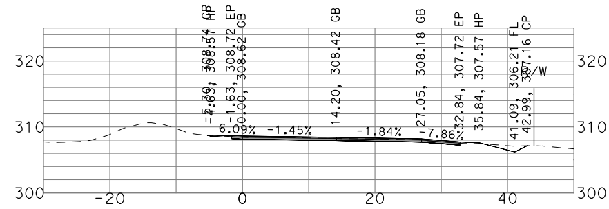
"GSB_R3_NB4" 526+00
