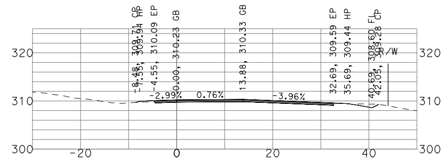
"GSB_R3_NB4" 449+00
