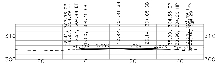
"GSB_R3_NB4" 484+00
