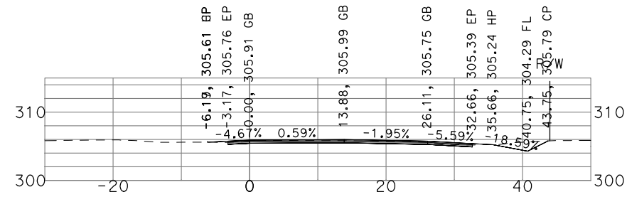
"GSB_R3_NB4" 505+00
