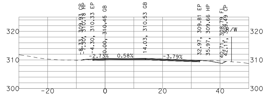
"GSB_R3_NB4" 447+50
