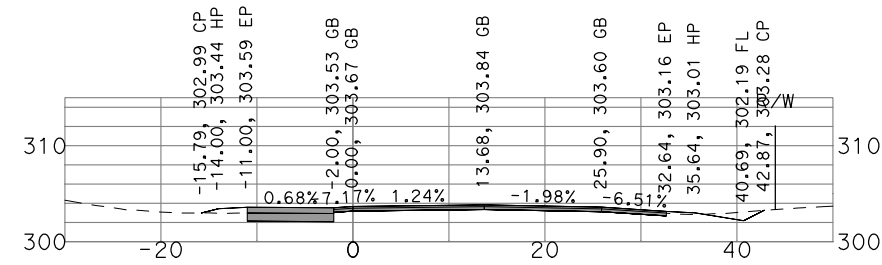
"GSB_R3_NB4" 497+50
