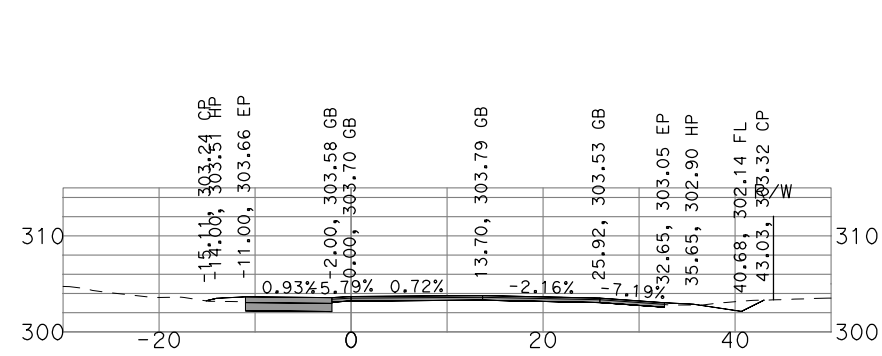
"GSB_R3_NB4" 498+00
