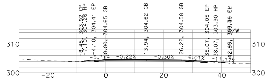
"GSB_R3_NB4" 483+50
