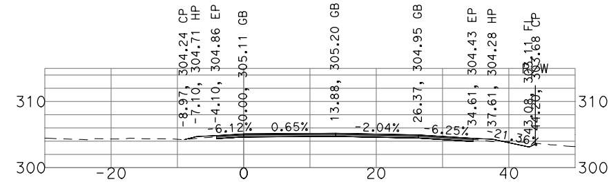
"GSB_R3_NB4" 485+00
