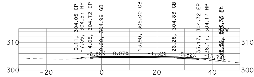
"GSB_R3_NB4" 484+50
