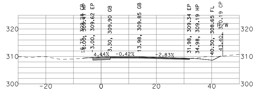
"GSB_R3_NB4" 465+50
