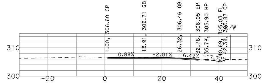
"GSB_R3_NB4" 506+50
