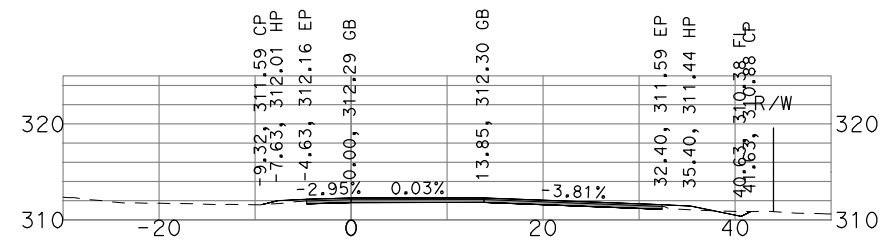
"GSB_R3_NB4" 453+00
