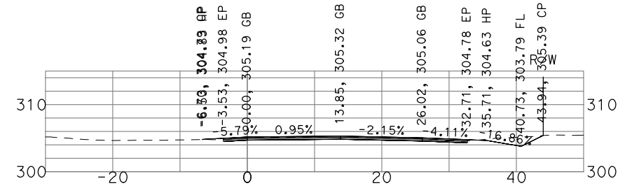
"GSB_R3_NB4" 503+50
