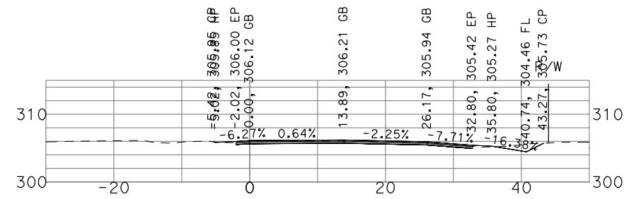
"GSB_R3_NB4" 505+50
