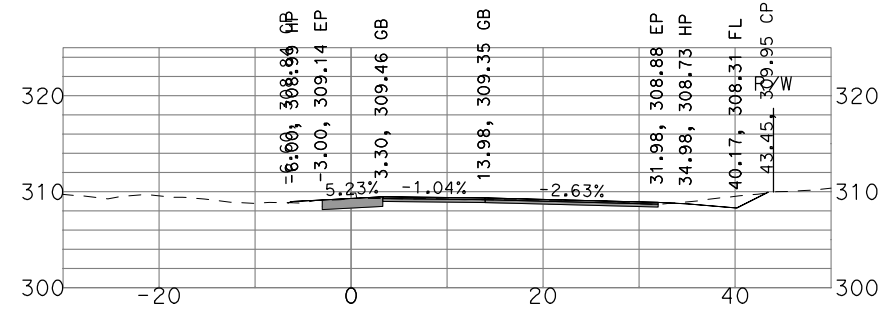
"GSB_R3_NB4" 466+00
