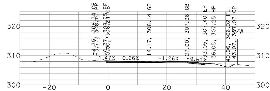
"GSB_R3_NB4" 527+00
