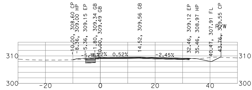
"GSB_R3_NB4" 538+00
