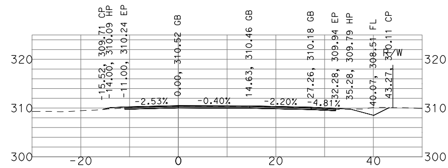
"GSB_R3_NB4" 540+00
