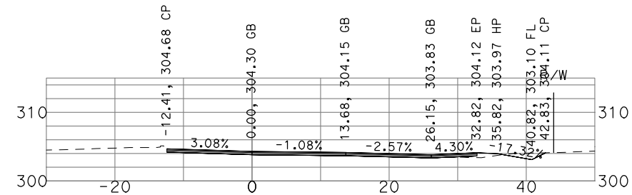
"GSB_R3_NB4" 494+00
