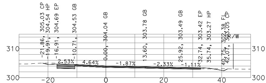
"GSB_R3_NB4" 495+50
