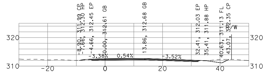
"GSB_R3_NB4" 453+50
