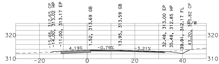
"GSB_R3_NB4" 459+50
