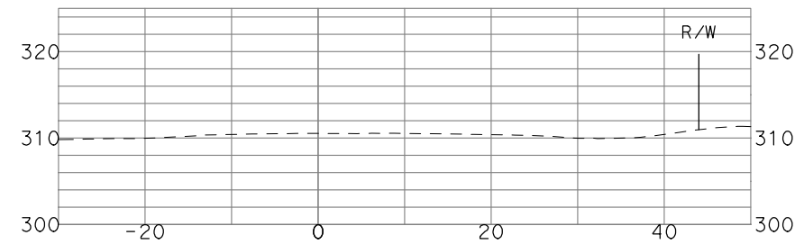
"GSB_R3_NB4" 542+00
