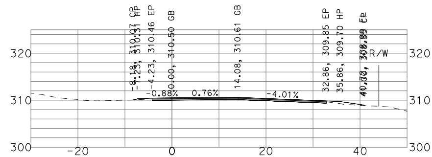
"GSB_R3_NB4" 447+00
