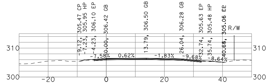
"GSB_R3_NB4" 490+00
