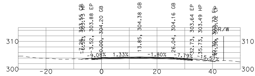
"GSB_R3_NB4" 501+50
