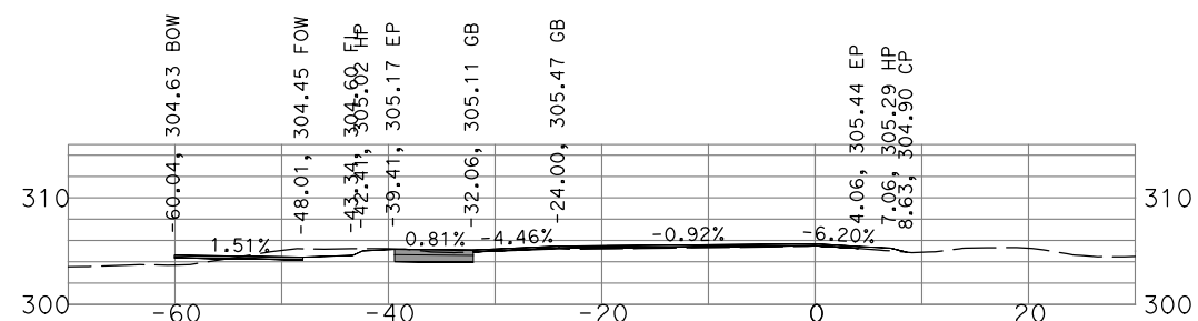
"GSB_R1_SB1" 93+50
