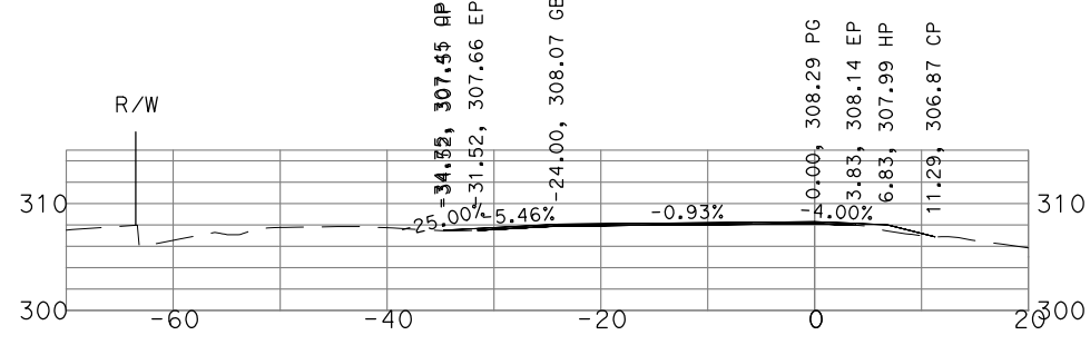
"GSB_R1_SB1" 160+00
