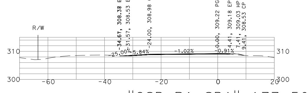
"GSB_R1_SB1" 177+50
