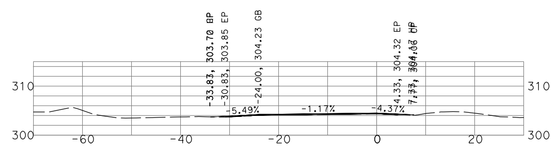
"GSB_R1_SB1" 112+50
