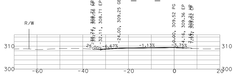
"GSB_R1_SB1" 185+00
