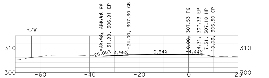
"GSB_R1_SB1" 152+00
