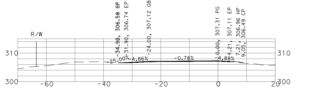
"GSB_R1_SB1" 150+00
