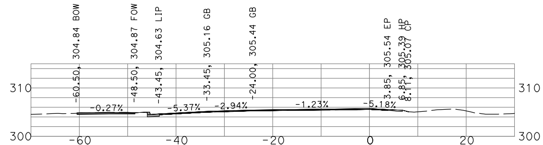
"GSB_R1_SB1" 95+00
