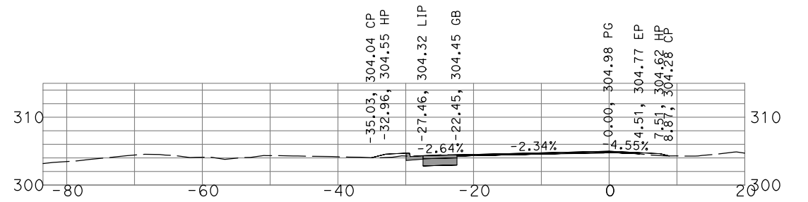
"GSB_R1_SB1" 81+50
