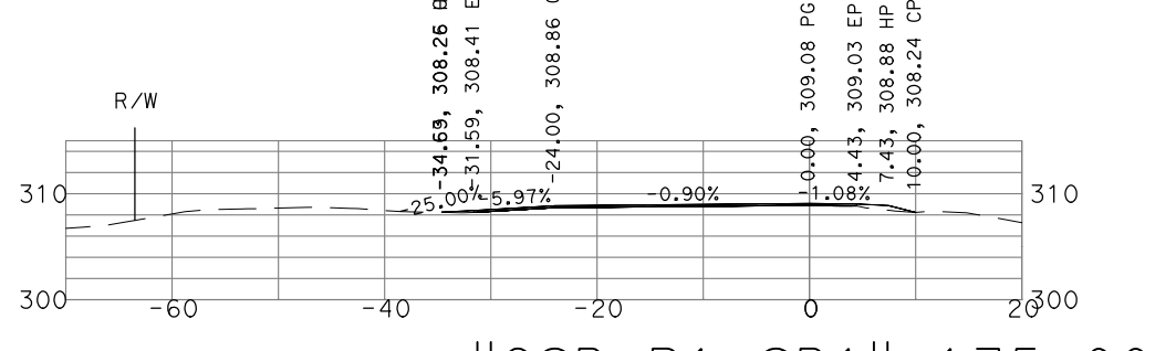
"GSB_R1_SB1" 175+00
