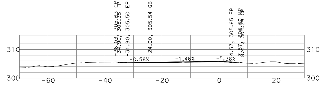
"GSB_R1_SB1" 98+00
