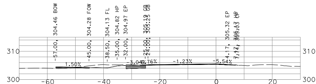
"GSB_R1_SB1" 92+00
