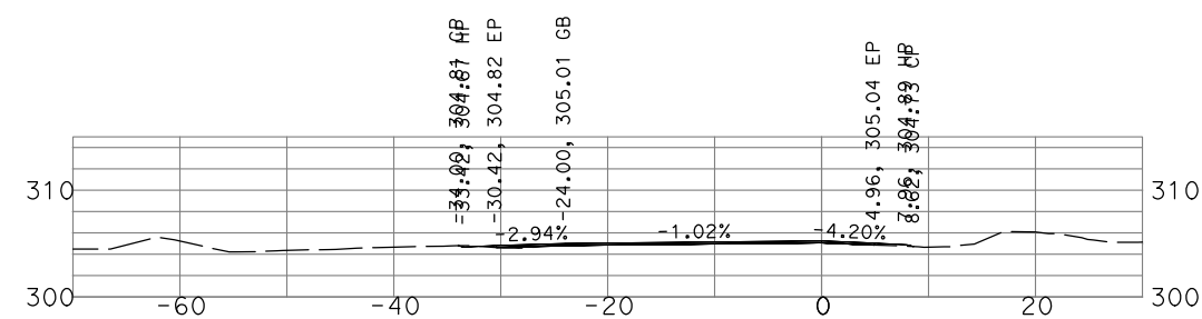
"GSB_R1_SB1" 111+00
