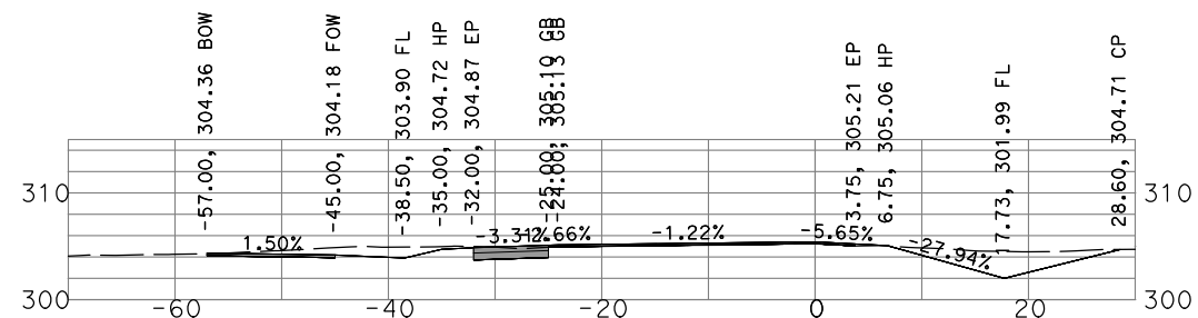
"GSB_R1_SB1" 90+50
