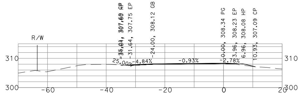
"GSB_R1_SB1" 161+00
