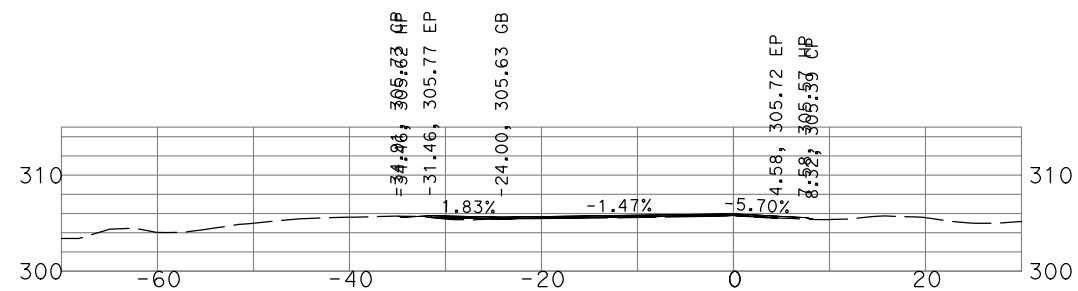
"GSB_R1_SB1" 98+50
