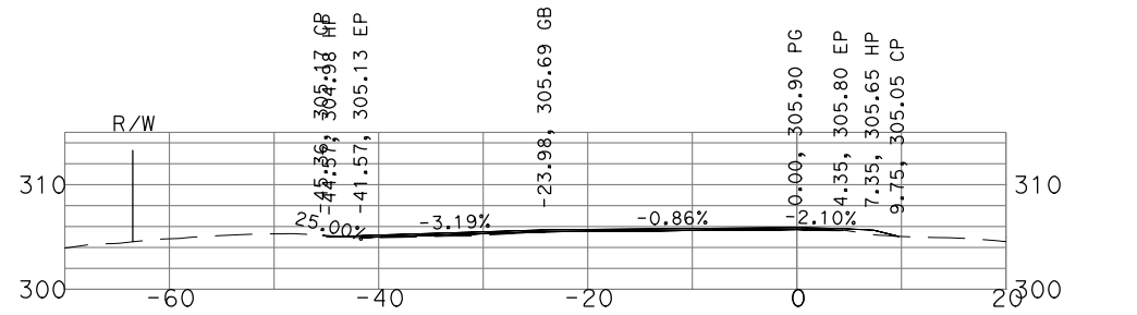
"GSB_R1_SB1" 135+00
