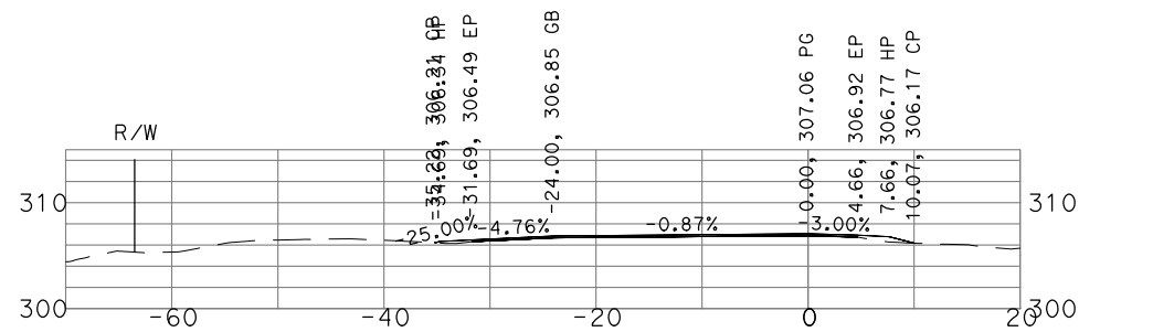
"GSB_R1_SB1" 147+00
