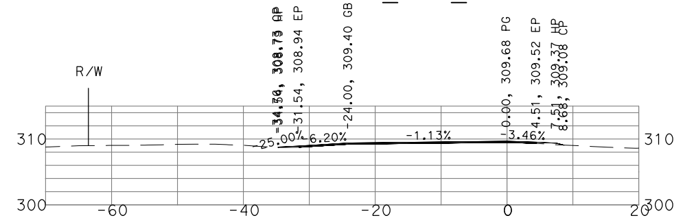
"GSB_R1_SB1" 188+50
