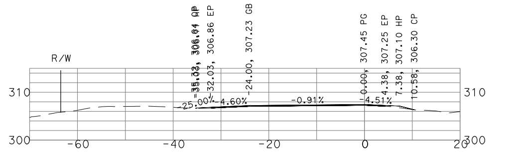
"GSB_R1_SB1" 151+50
