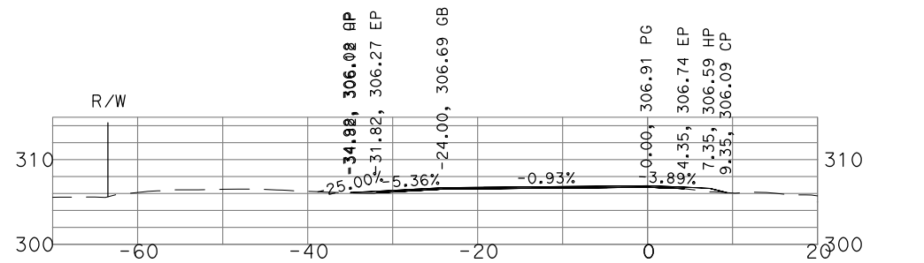
"GSB_R1_SB1" 145+50
