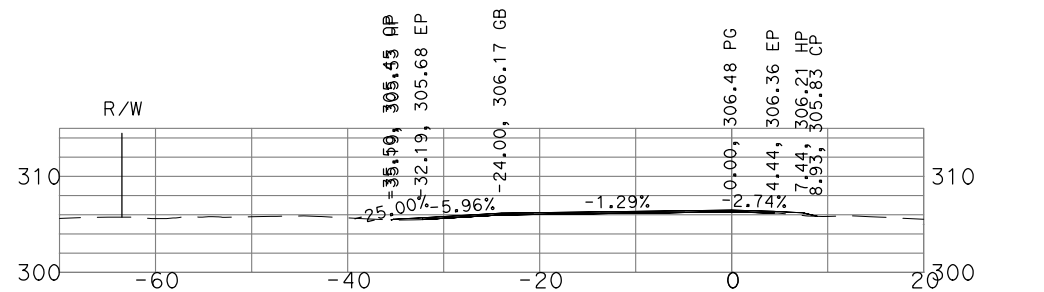
"GSB_R1_SB1" 141+00
