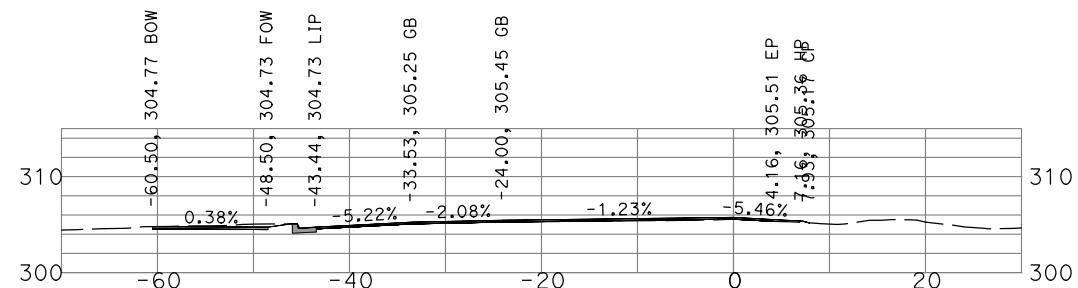
"GSB_R1_SB1" 94+50
