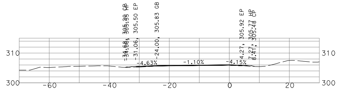
"GSB_R1_SB1" 108+50
