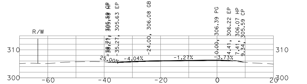
"GSB_R1_SB1" 139+50
