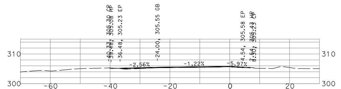
"GSB_R1_SB1" 97+50
