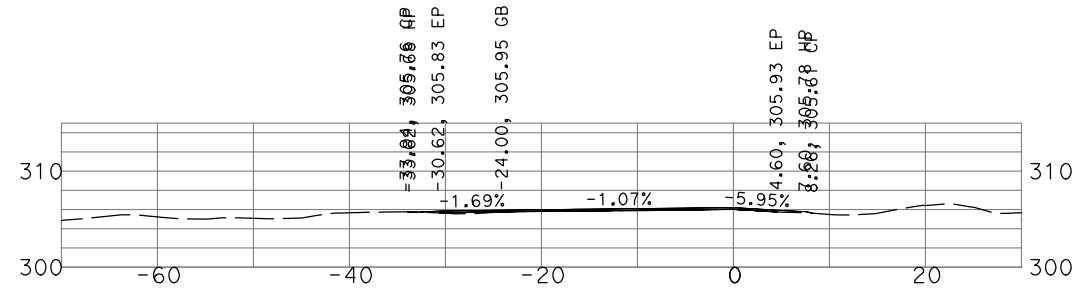
"GSB_R1_SB1" 103+50
