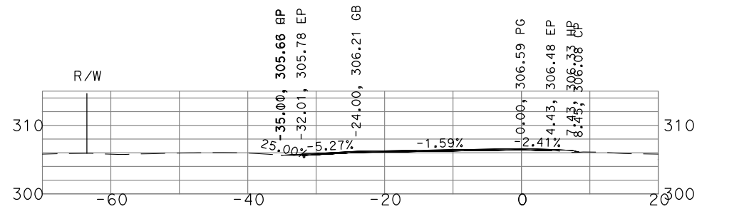
"GSB_R1_SB1" 142+00
