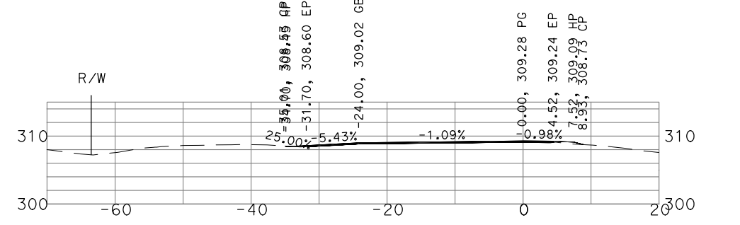
"GSB_R1_SB1" 179+00
