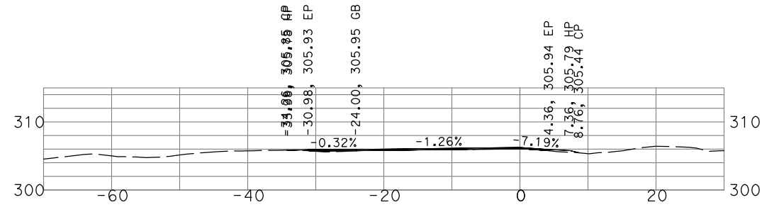
"GSB_R1_SB1" 104+00
