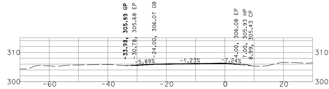
"GSB_R1_SB1" 106+50
