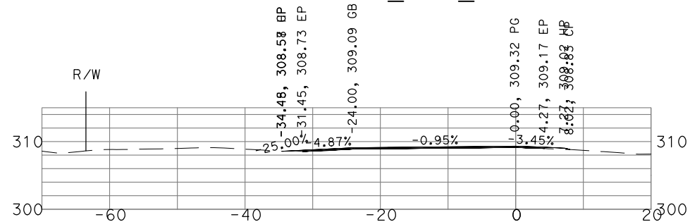
"GSB_R1_SB1" 181+00
