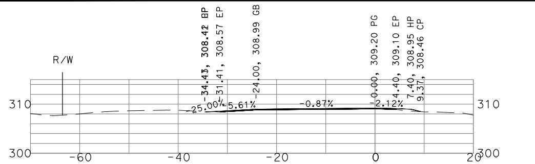
"GSB_R1_SB1" 177+00
