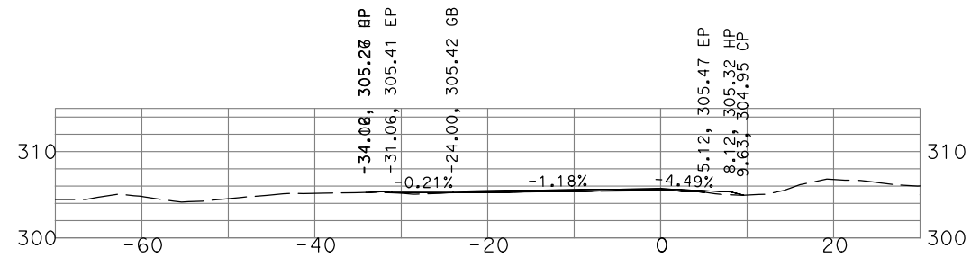
"GSB_R1_SB1" 110+00
