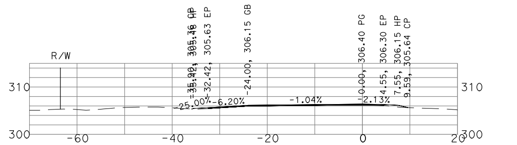
"GSB_R1_SB1" 140+00
