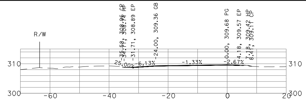
"GSB_R1_SB1" 189+50
