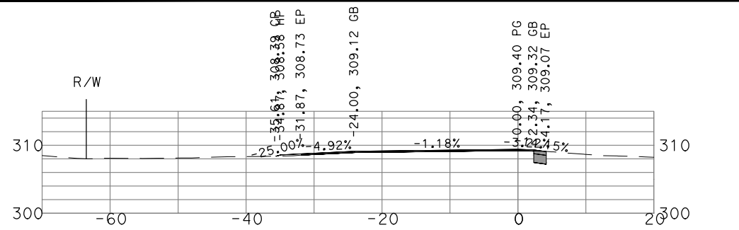
"GSB_R1_SB1" 182+00
