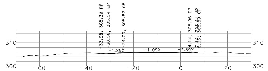
"GSB_R1_SB1" 101+00
