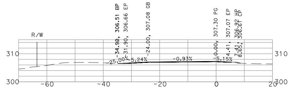
"GSB_R1_SB1" 149+50
