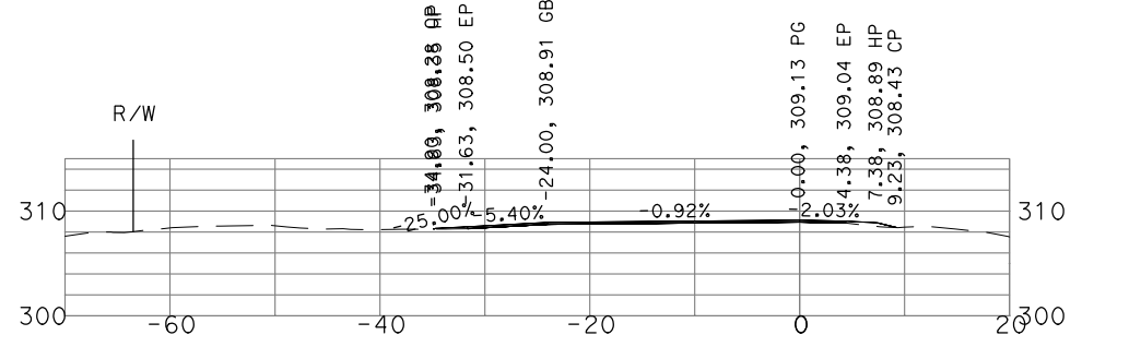
"GSB_R1_SB1" 176+00
