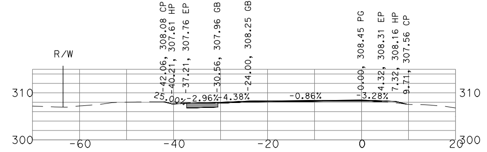
"GSB_R1_SB1" 163+00
