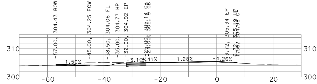
"GSB_R1_SB1" 91+50
