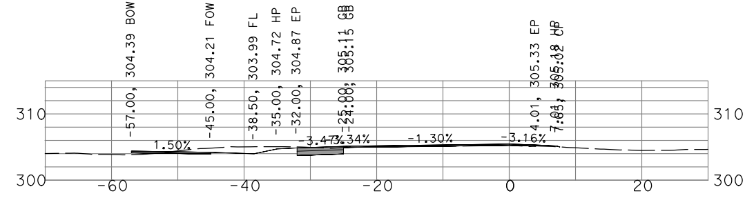
"GSB_R1_SB1" 91+00
