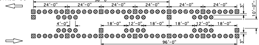
DETAIL 35
