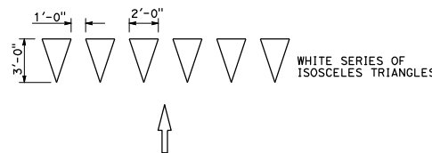
YIELD LINE
