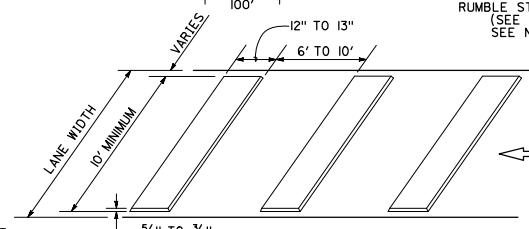
PORTABLE TRANSVERSE RUMBLE STRIP ARRAY DETAIL
