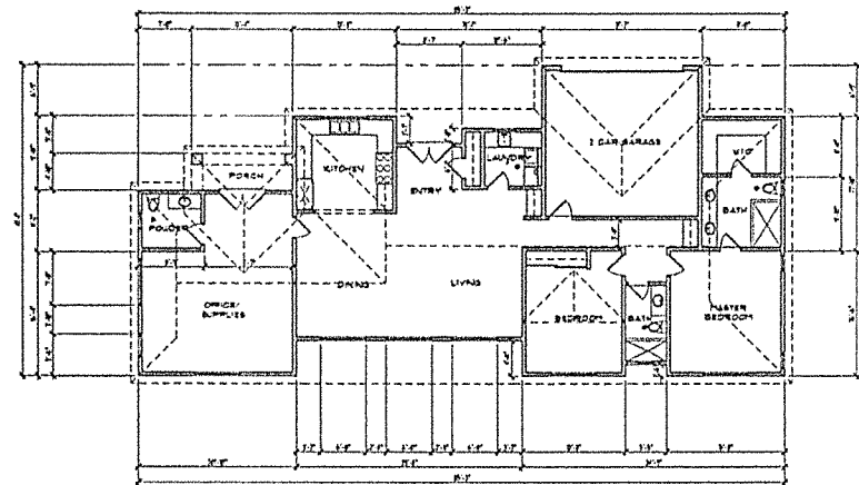
① FLOOR PLAN - BUILDING 1
