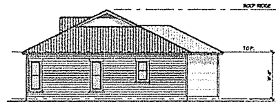
③ RIGHT SIDE ELEVATION 1/8" = 1'-0"
